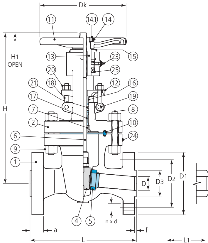
WCB, LCC: NPS 2" - 4" Chrome Alloy: NPS 2" - 6"
