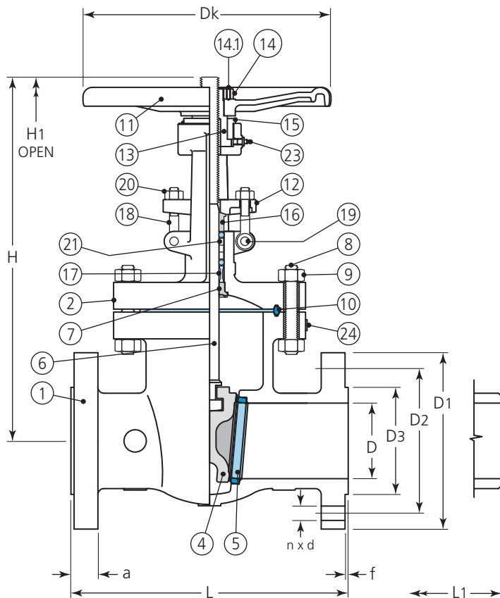
WCB, LCC: NPS 2"-6" Chrome Alloy: NPS 2"-8"
