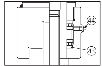
Yoke Sleeve Detail with Ball Bearing WCB, LCC: NPS 8" Only Chrome Alloy: NPS 8" Only
