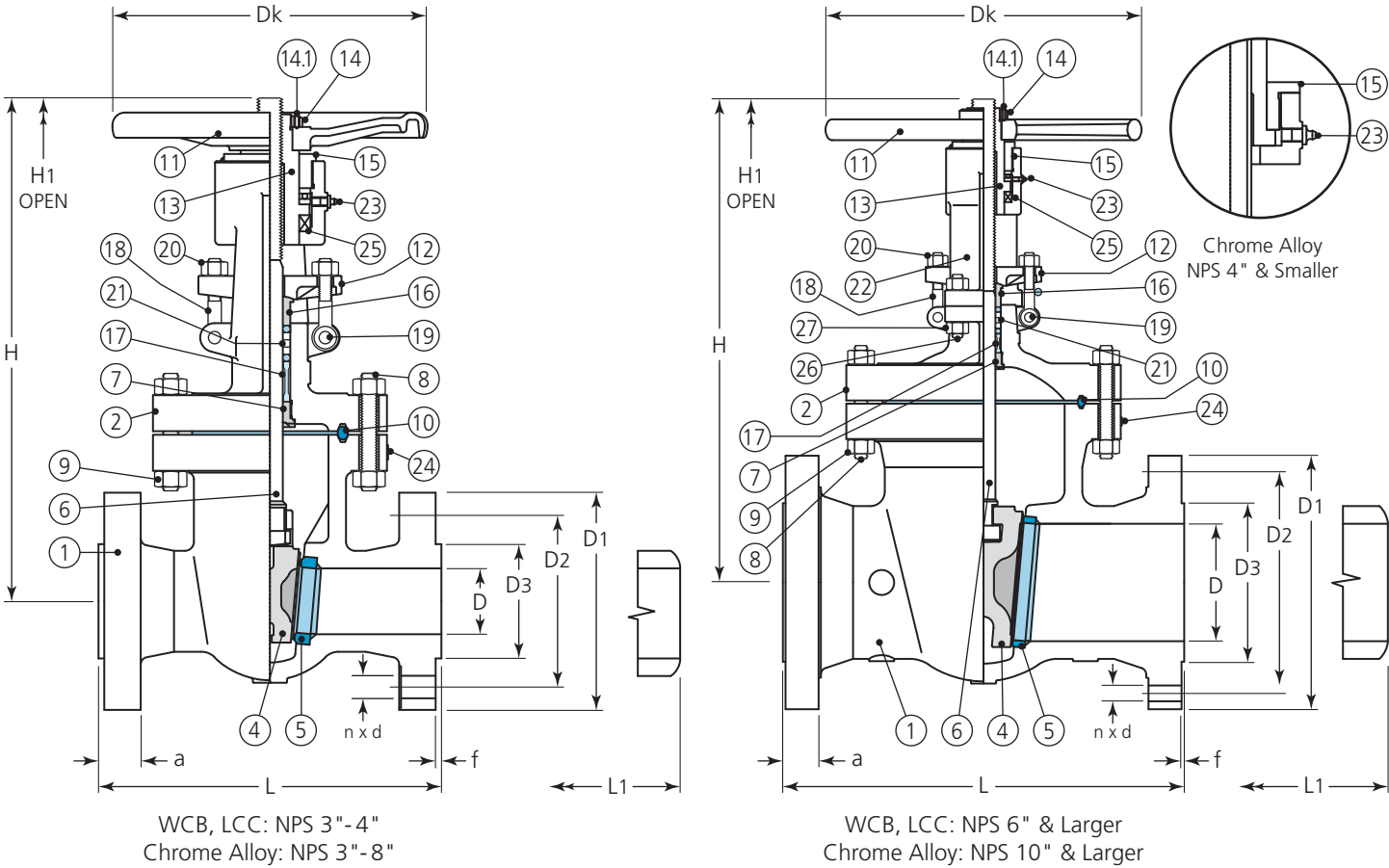
Dimensional Data (in.) & Flow Coefficient (Cv)
