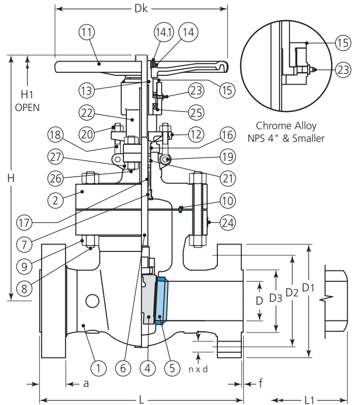
WCB, LCC: NPS 6" & Larger Chrome Alloy: NPS 8" & Larger
